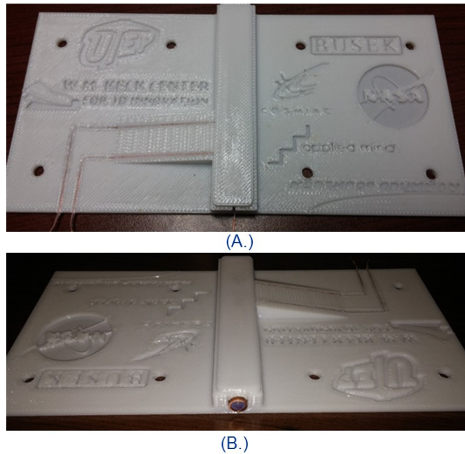
Figure 13: Photographs of embedded \mu PPT thrusters. (A.) Top view (B.) Thruster end view
